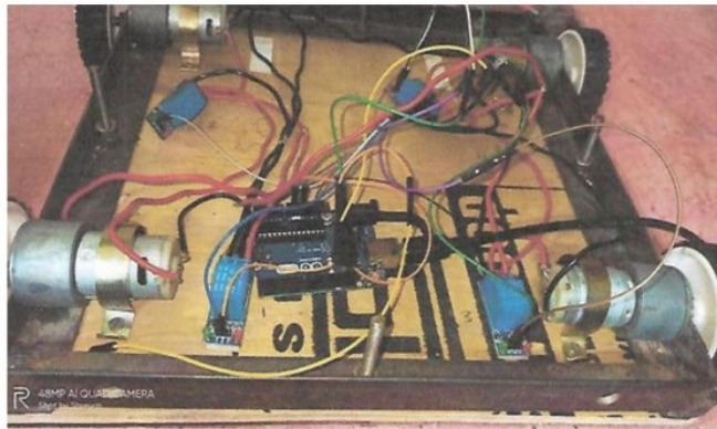
CRD Base with Circuit connections
